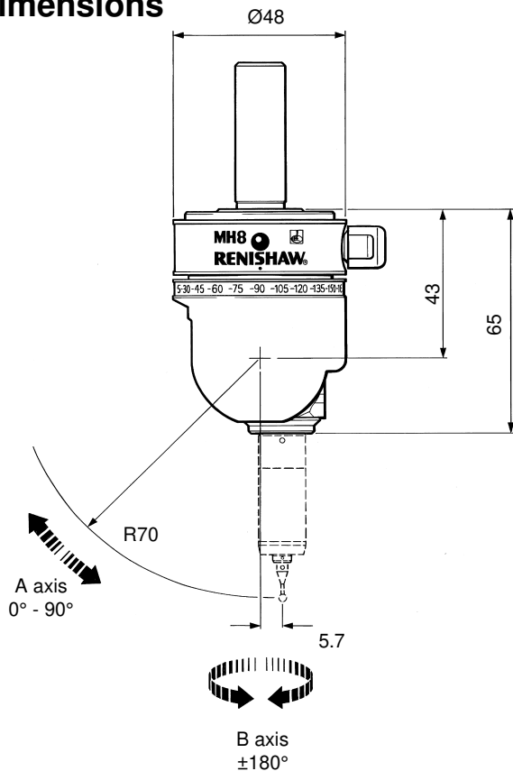
Figure 5 - MH8 dimensions
