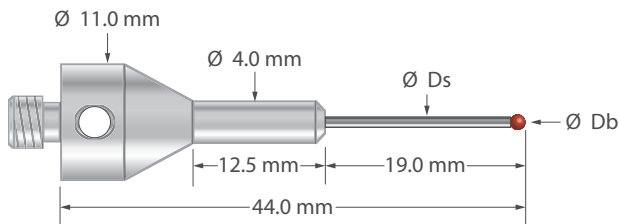
M5 stylus with ball, carbide stem and 11.0 mm diameter x 25.0 mm long stainless steel base.
