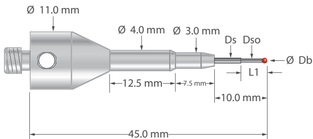
M5 stylus with ball, carbide stem, and 11.0 mm diameter x 25.0 mm long stainless steel base.
