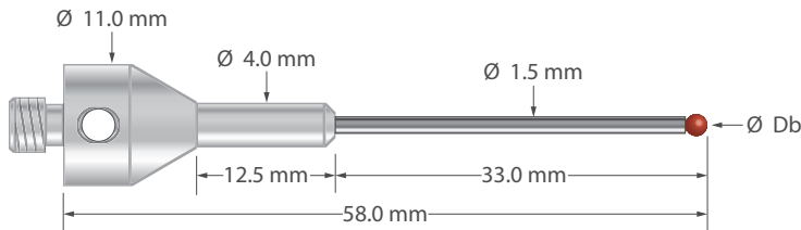
M5 stylus with ball, carbide stem, and 11.0 mm diameter x 25.0 mm long stainless steel base.
