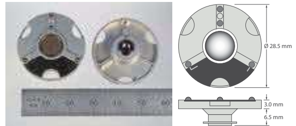
M3 adapter plate, aluminum, with ID chip. Fits TL3 probe head.
