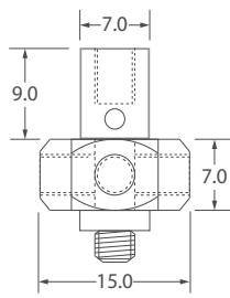
M4 5-way hub. Fully adjustable, two-piece assembly. Stainless steel.
