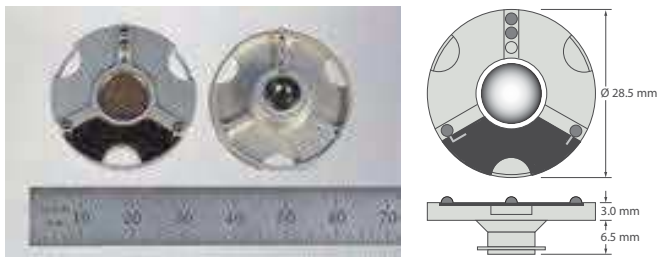
M3 adapter plate, aluminum, with ID chip. Fits TL1 probe head.
