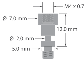
"Weak Link" with M4 male and M4 female threads. Machined from SAE 4140 chromoly steel. Black oxide finish.
