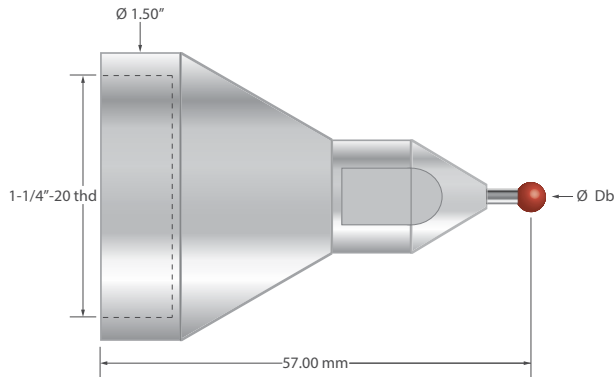
Faro compatible stylus with carbide stem and stainless steel base.
