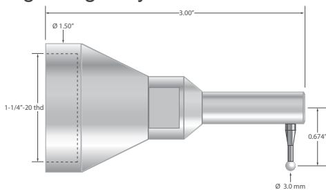
Faro compatible right angle stylus with stainless steel base, carbide stem, and 3.0 mm diameter zirconia ball.
