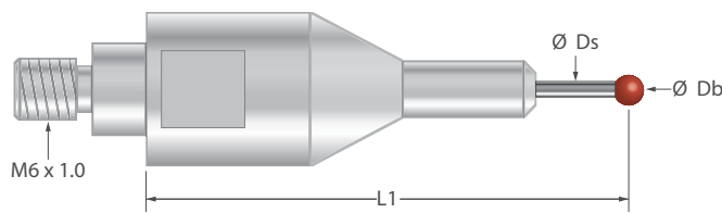
Faro compatible stylus with carbide stem and stainless steel base.
